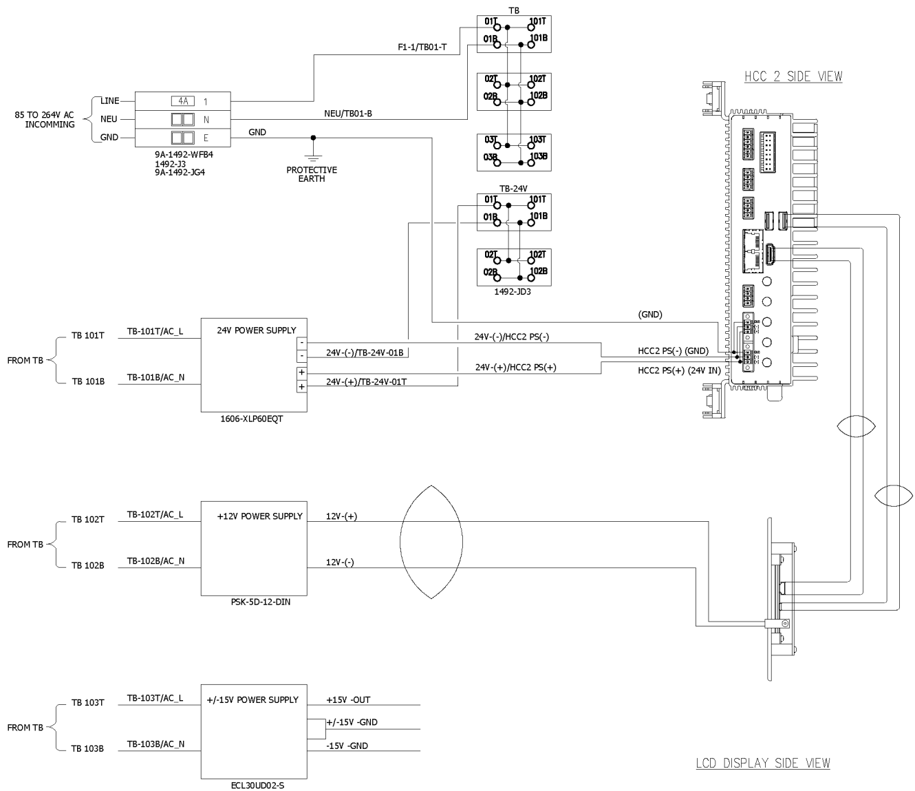
Figure D.3—HCC2 power and display wiring details
