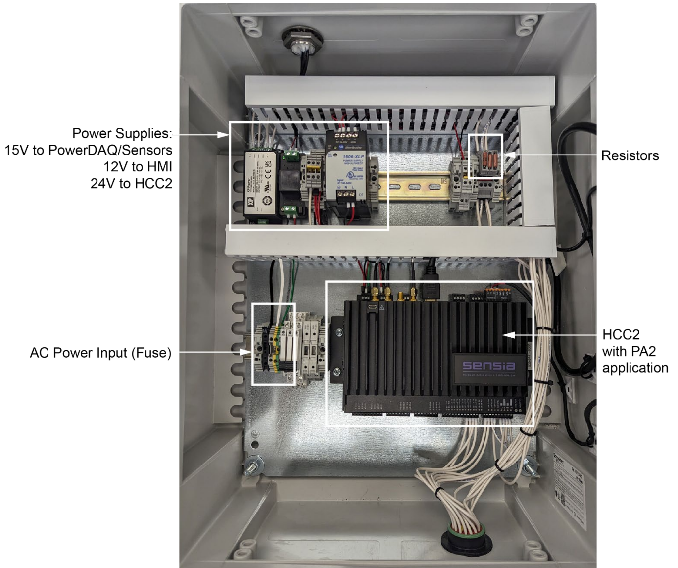
Figure 4.2—Controller cabinet components
