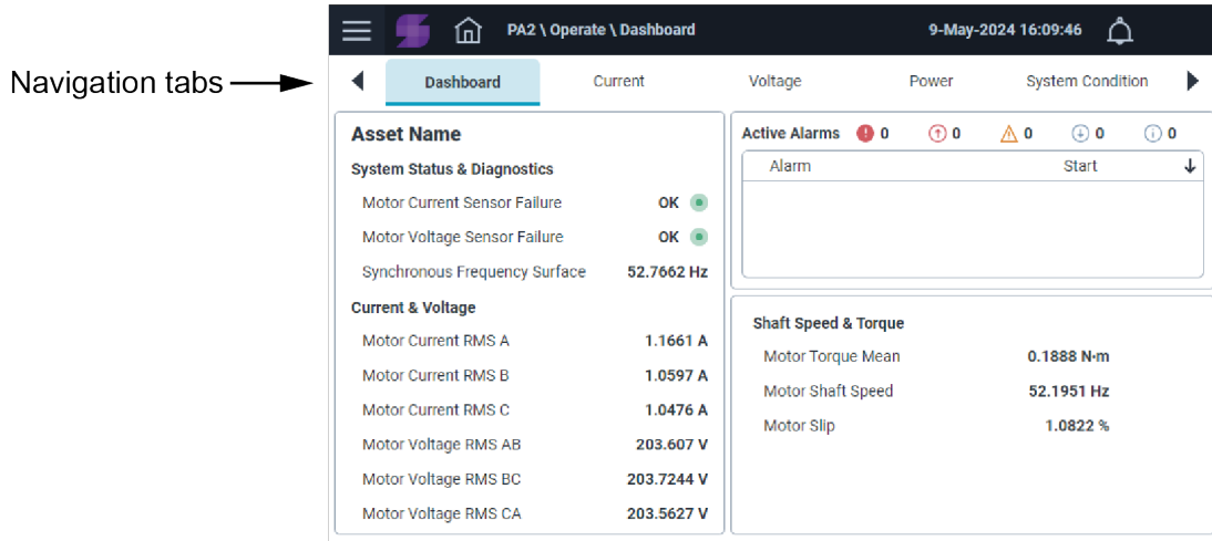
Figure 7.5: Navigation Tabs
