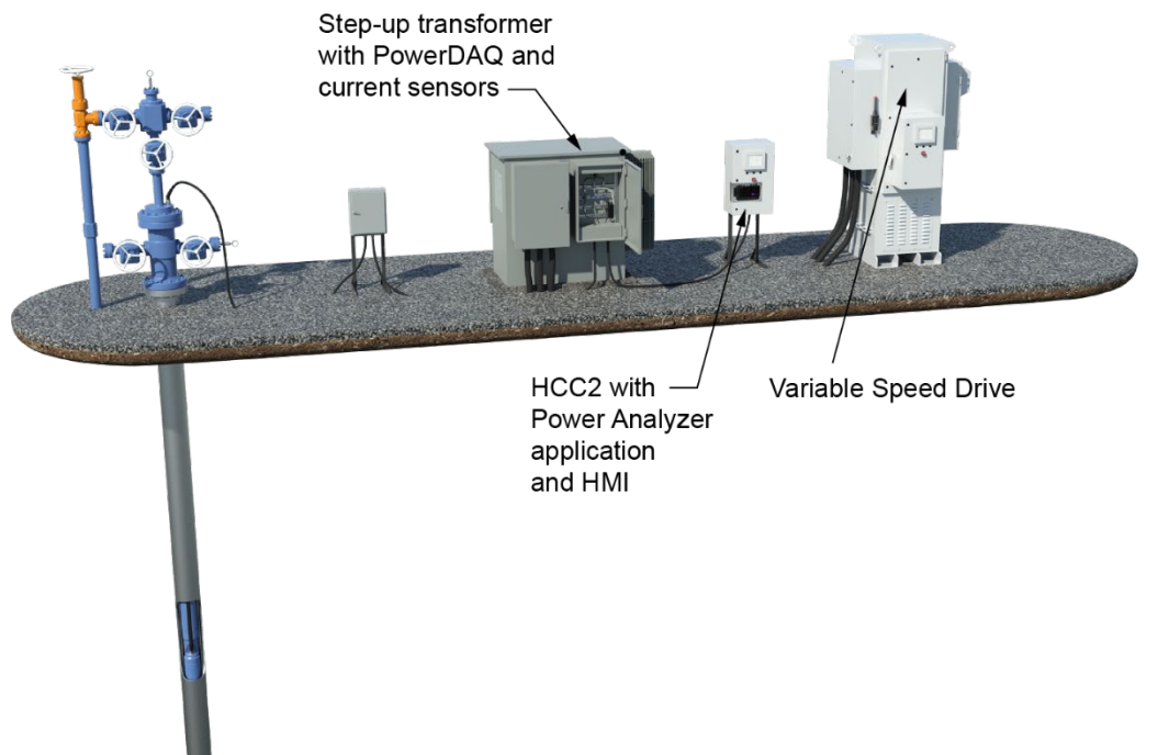
Figure 2.1—Typical INSTRUCT Power Analyzer 2.0 wellsite installation
