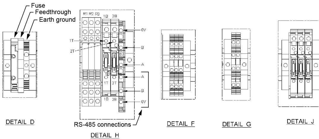
Figure D.2—HCC2 controller backplane layout
