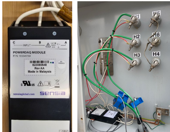
Figure 4.8—PowerDAQ voltage cable (left) and output phase (right) connections
