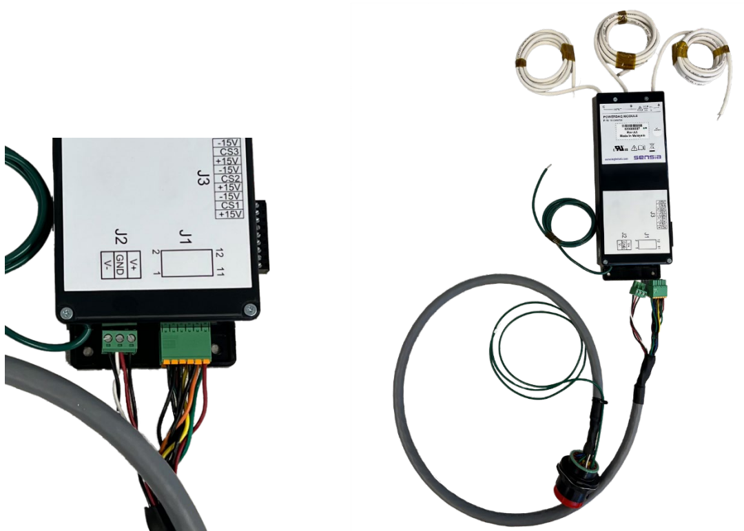
Figure 4.12—Cable connects PowerDAQ to HCC2 for transmission of analog input signals and power
