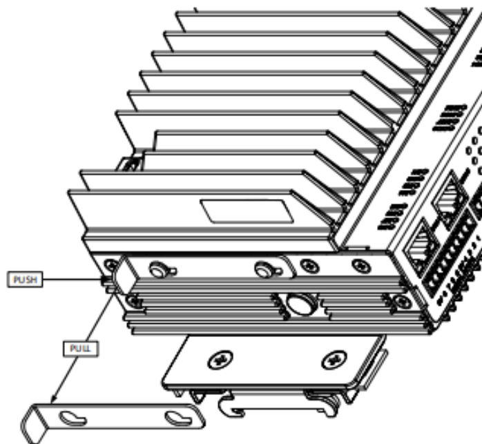
Figure 4.14—HCC2 microSIM card access
