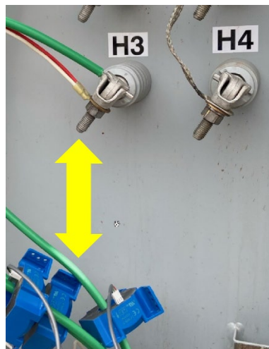
Figure 4.6—Required separation of sensors from transformer bushings
