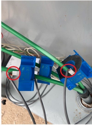
Figure 4.7—PowerDAQ to current sensor connections
