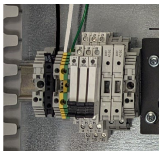
Figure 4.3—AC Power Connection in HCC2 Cabinet
