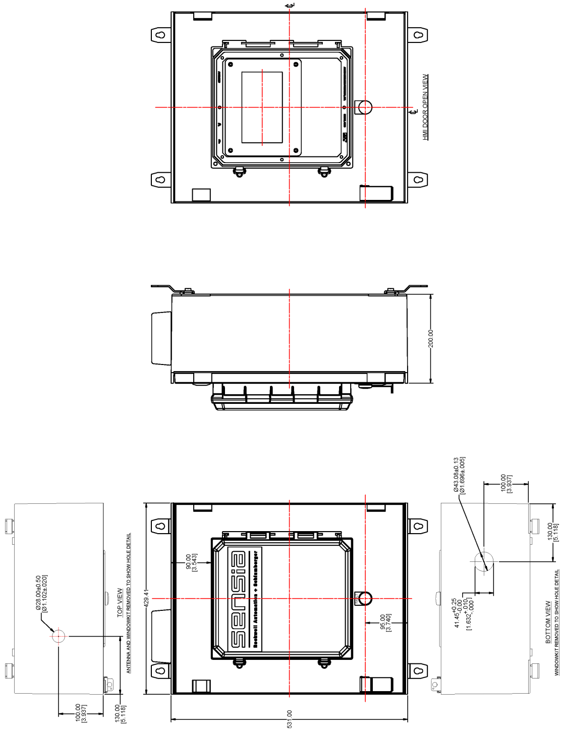
Figure D.1—HCC2 controller cabinet dimensions
