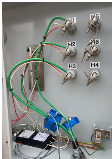
Figure 4.4—PowerDAQ in secondary (load) side of transformer cabinet
